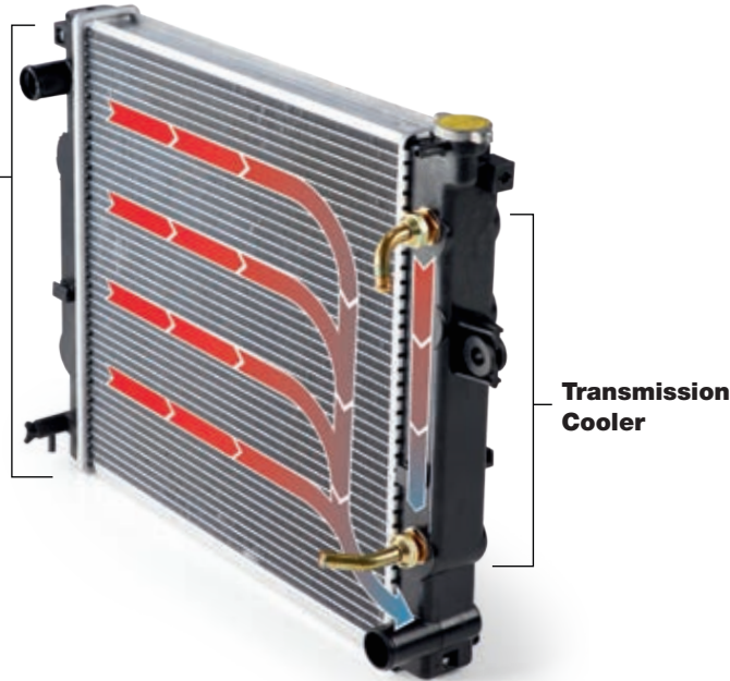
Engine Radiator
