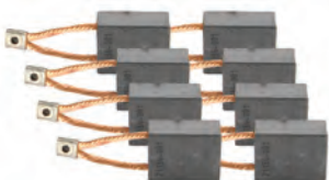
Part Number - 116961 Brush Set (Set of 8) 0.628 D x 1.247 W x 1.500 L
