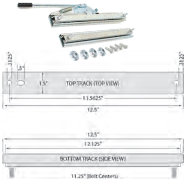
Part Number - 380030-265 Seat Tracks
