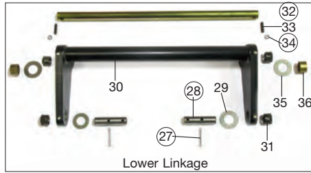
Lower Linkage
