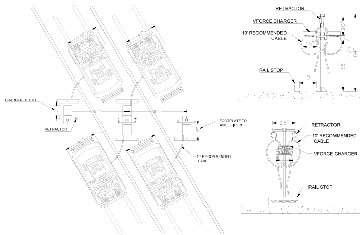
FC PUF DIAGONAL (Back to Back)
