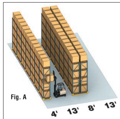
Selective Rack Counterbalanced Lift Truck
