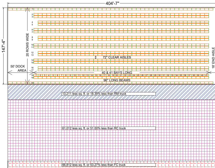
TSP - TURRET TRUCK LAYOUT 32' CLEAR HEIGHT - 6 PALLETS HIGH, 826 BAYS OF RACK, 9,912 PALLET POSITIONS BUILDING= 58,609 SQUARE FEET, 5.9 SQ. FT. PER PALLET POSITION
