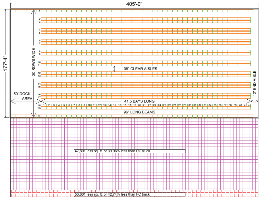
RM - REACH TRUCK LAYOUT 32' CLEAR HEIGHT - 6 PALLETS HIGH, 825 BAYS OF RACK, 9,900 PALLET POSITIONS BUILDING= 71,820 SQUARE FEET, 7.3 SQ. FT. PER PALLET POSITION
