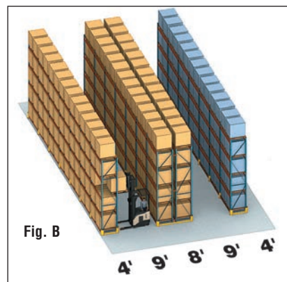
Selective Rack Rider Reach Truck 33% more storage over Fig. A
