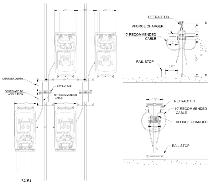
FC PUF (Back to Back)
