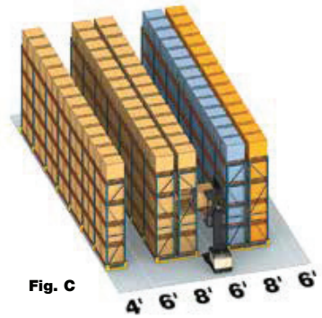
Selective Rack Turret Stockpicker 25% more storage over Fig. B 66% more storage over Fig. A
