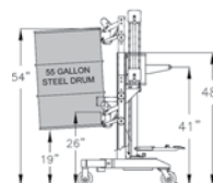
DM-1100 - 240150 STANDARD LIFT
