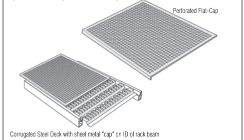
Open Area Accessory, Perforated Flat-Cap
