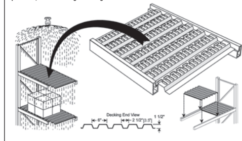
Open Area, Water Drainage Decking
