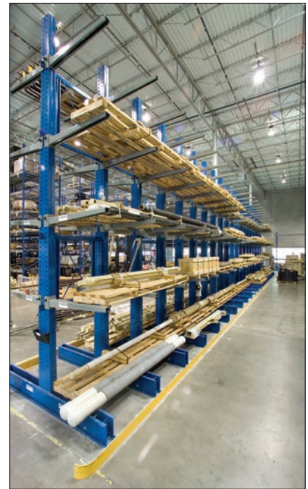
Cantilever Rack
