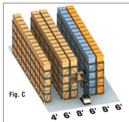
Selective Rack Turret Stockpicker 25% more storage over Fig. B; 66% more storage over Fig. A
