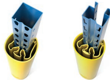
Rack Bull XL for 3" deep uprights
