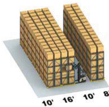
Double-Deep Rack Double Reach Lift Truck 8.5'-11' aisle width
