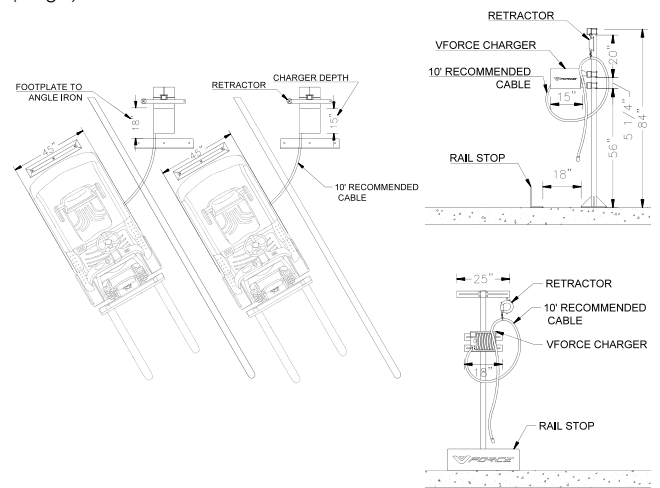
FC PUF DIAGNAL (Single)
