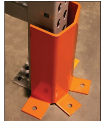
Floor Mounted Column Protector
